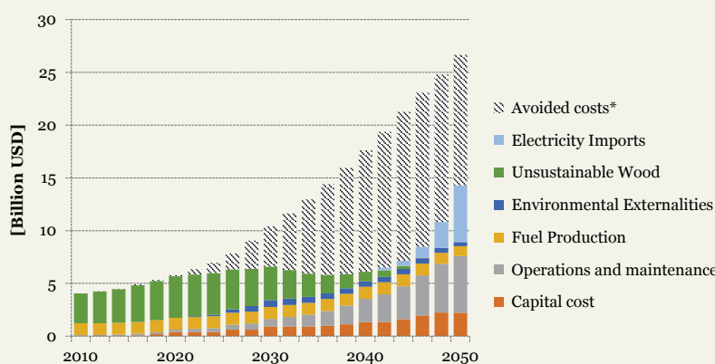
Figure 6: Costs associated with the renewable energy scenario Uganda including avoided costs as compared to the reference energy scenario
