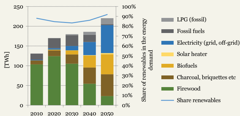
Figure 36: Energy demand in Uganda (bars) and the share of renewables in the energy system (line) – renewable energy scenario
